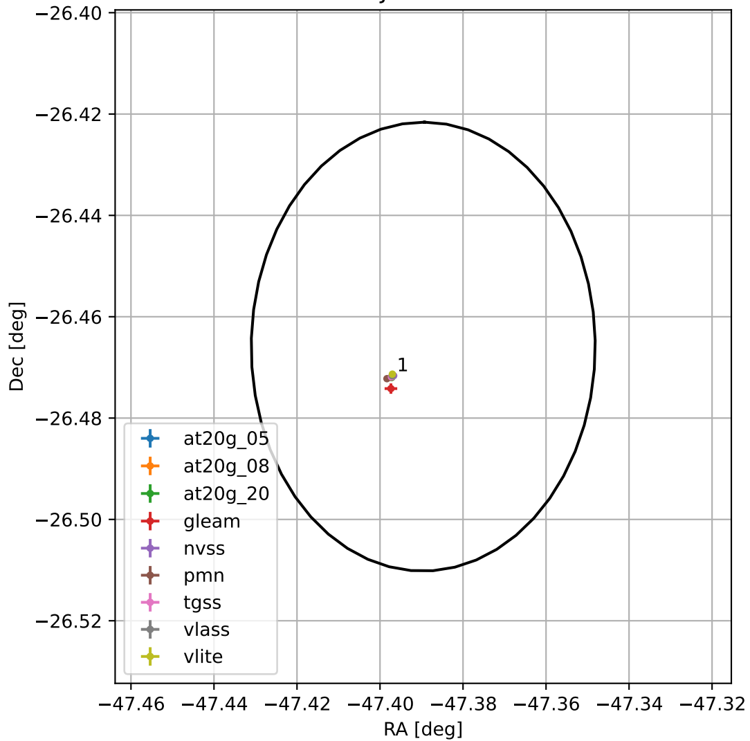
4FGL J2050.4-2627
