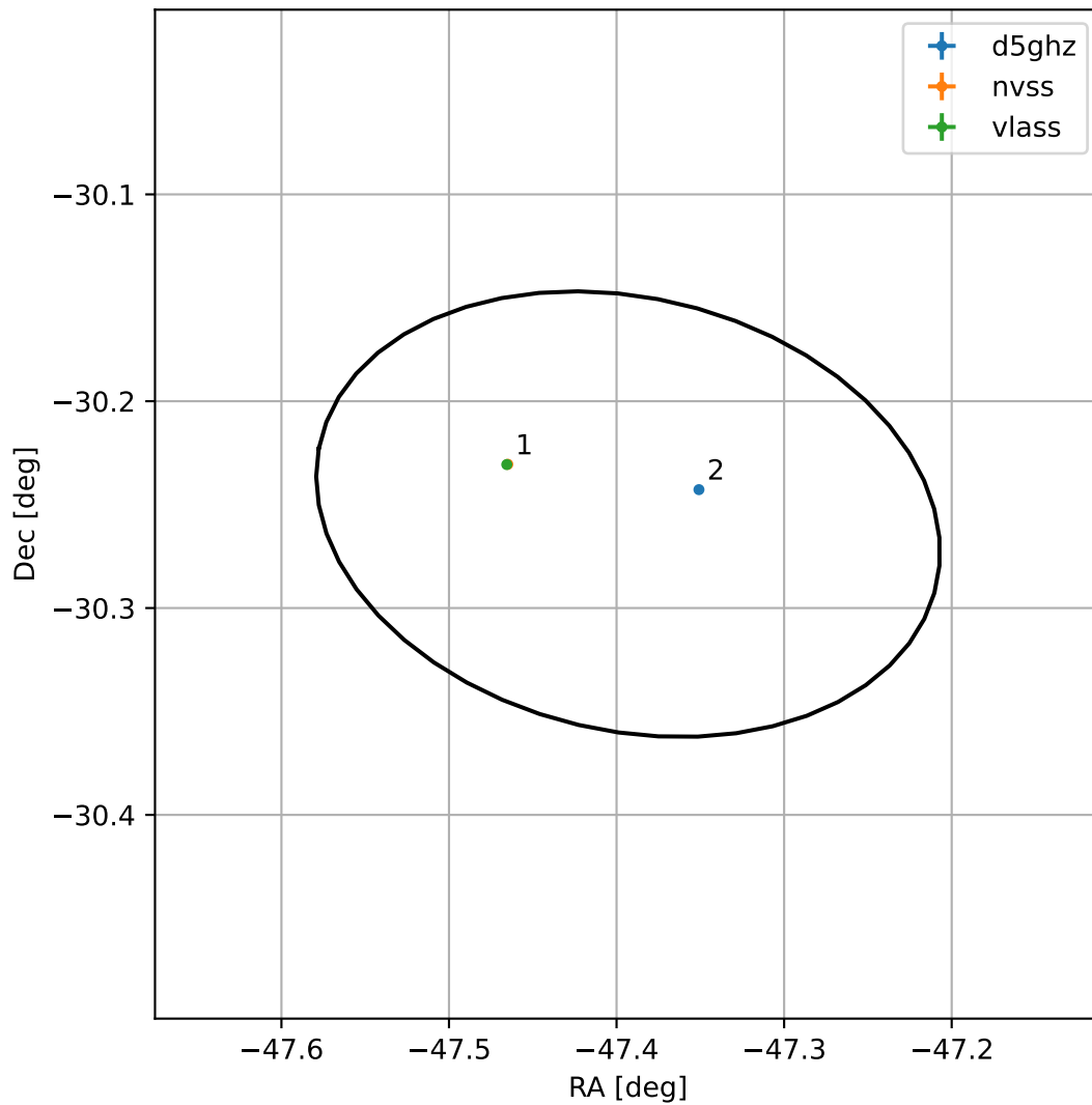
4FGL J2050.4-3015
