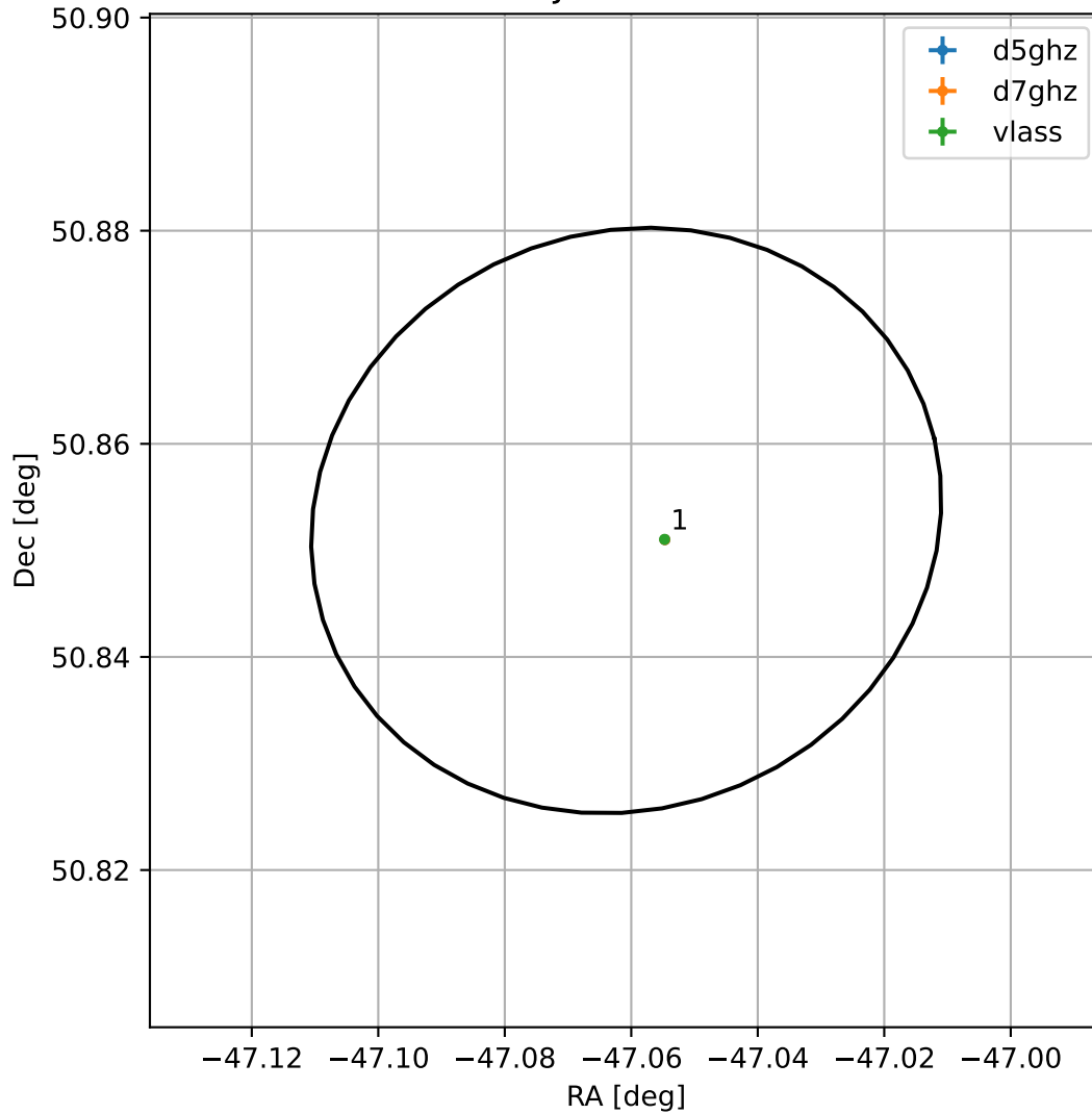
4FGL J2051.7+5051
