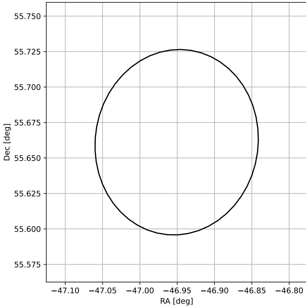
4FGL J2052.1+5539
