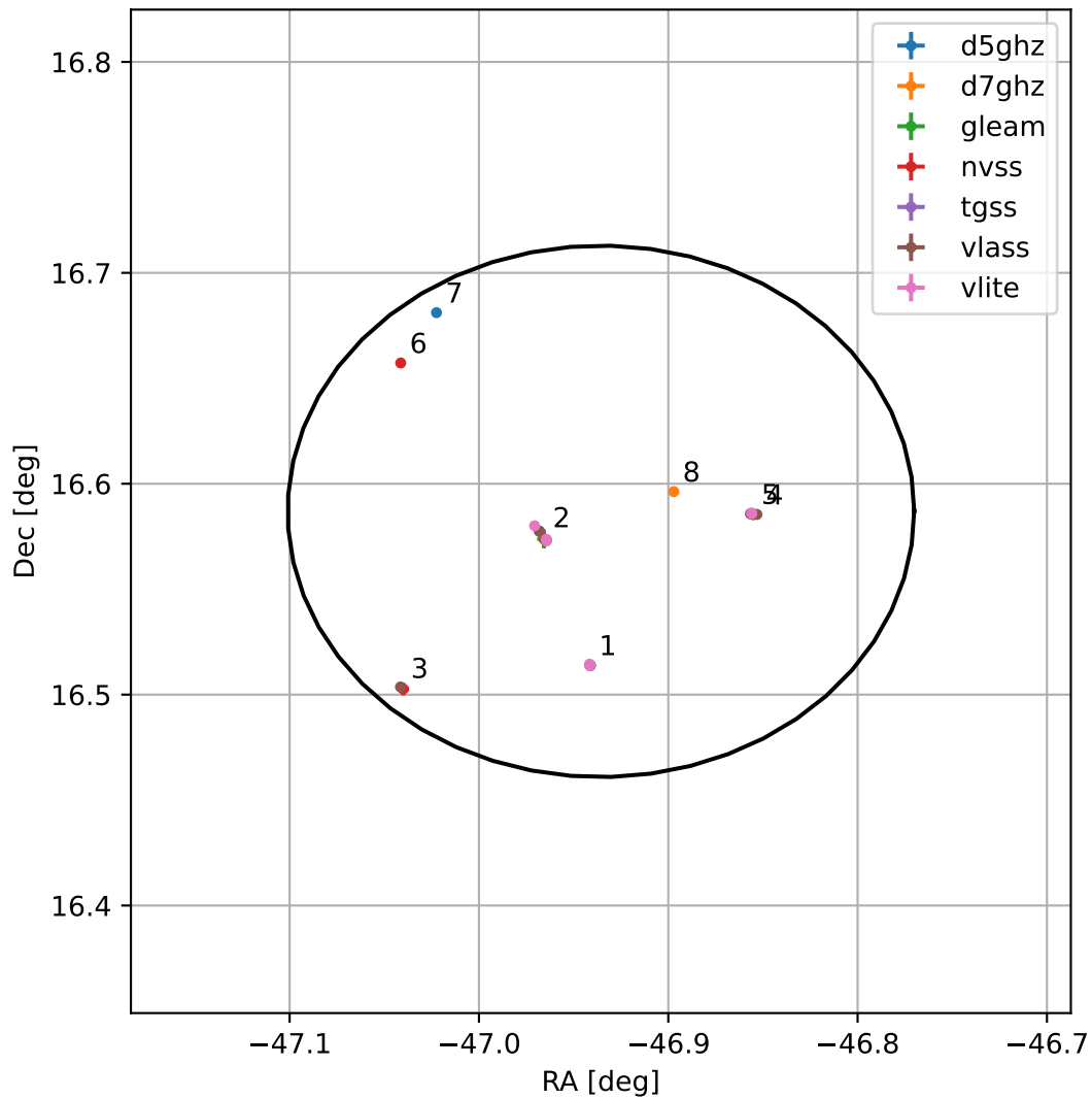
4FGL J2052.2+1635
