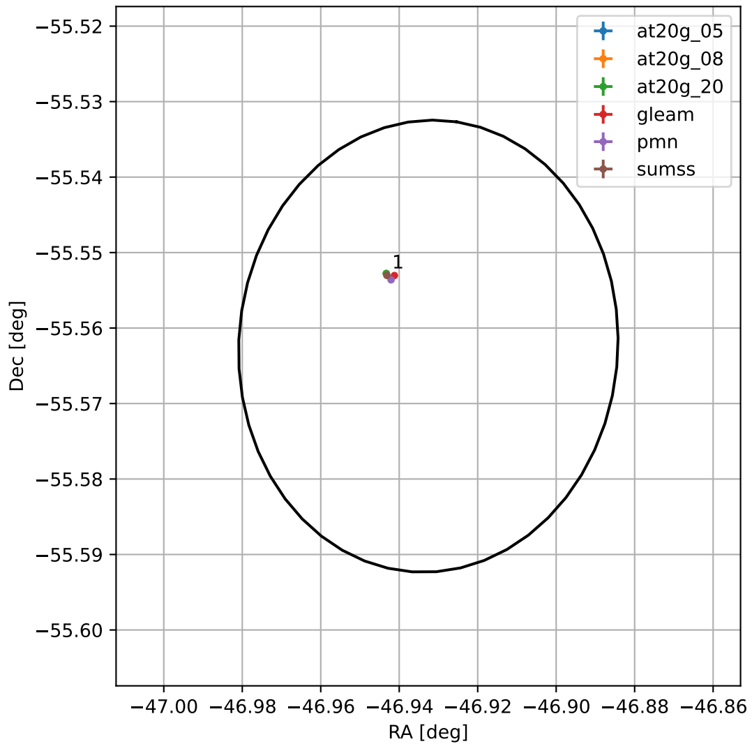
4FGL J2052.2-5533
