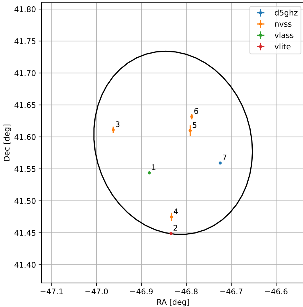
4FGL J2052.6+4135
