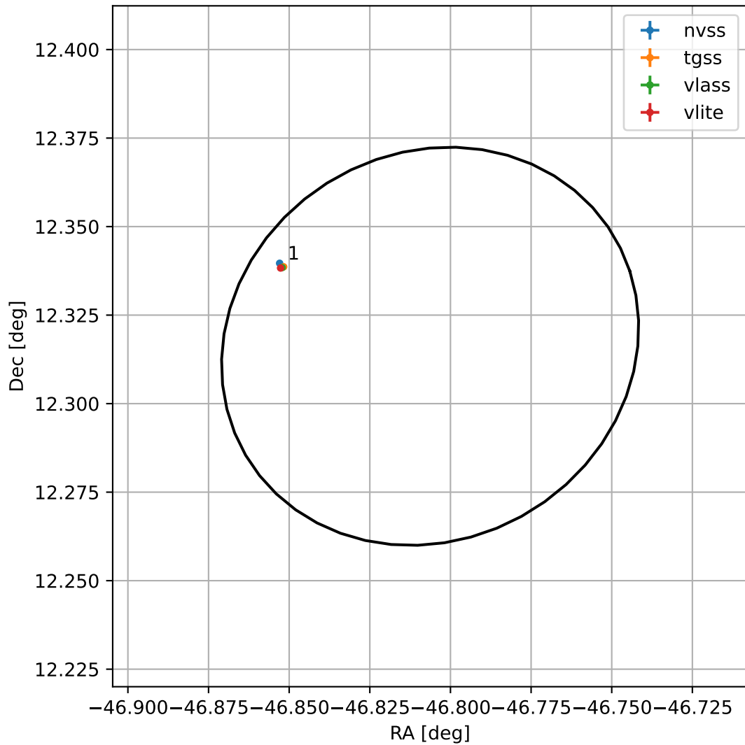
4FGL J2052.7+1218
