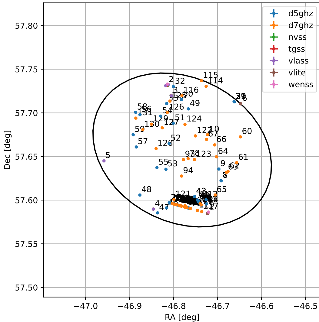
4FGL J2052.8+5739
