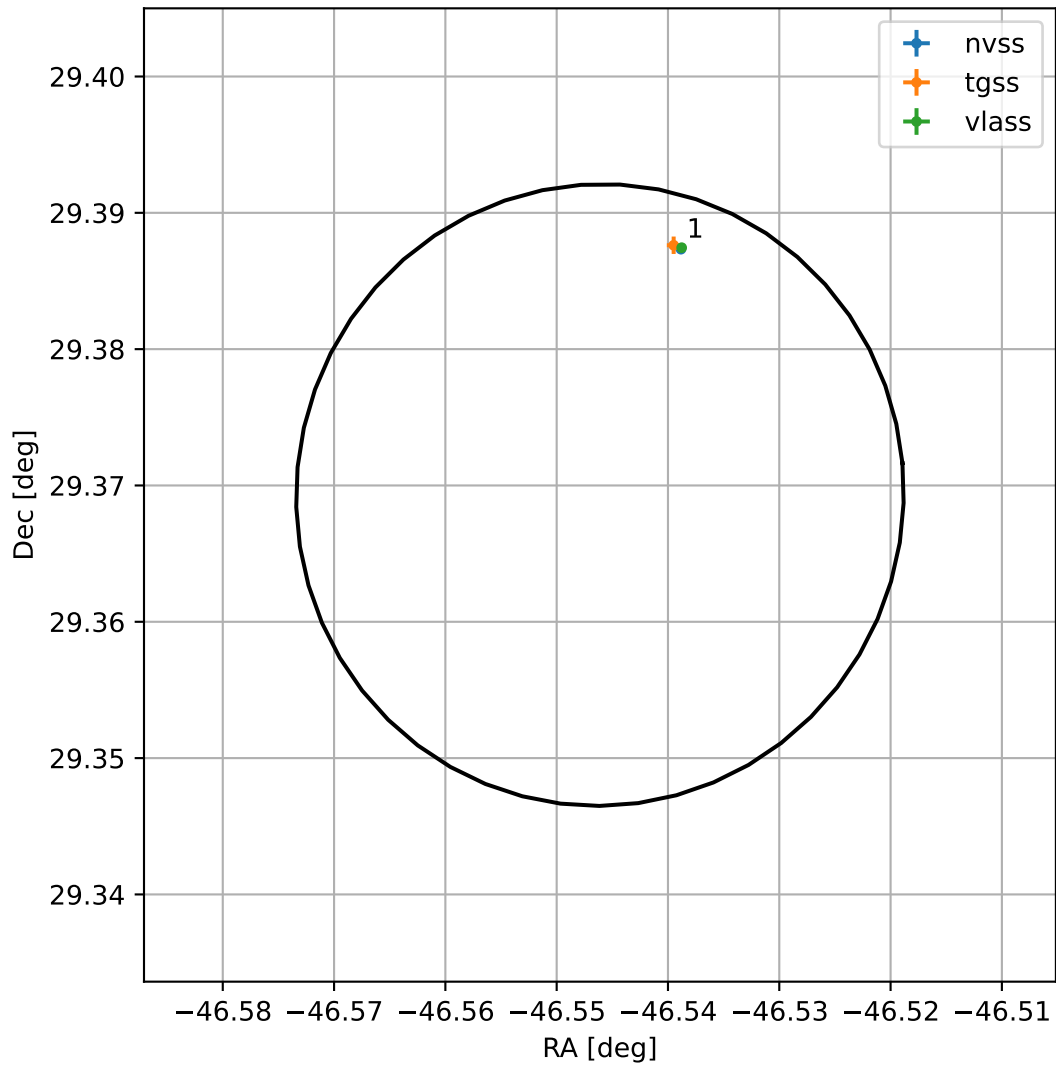
4FGL J2053.8+2922
