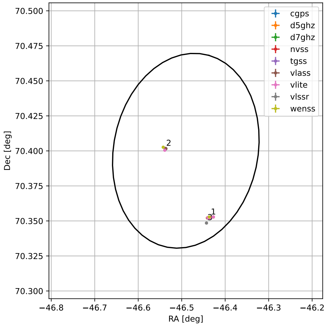
4FGL J2054.0+7024
