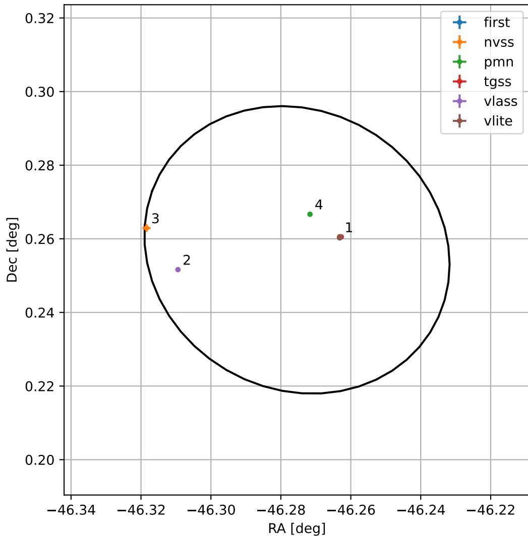
4FGL J2054.8+0015
