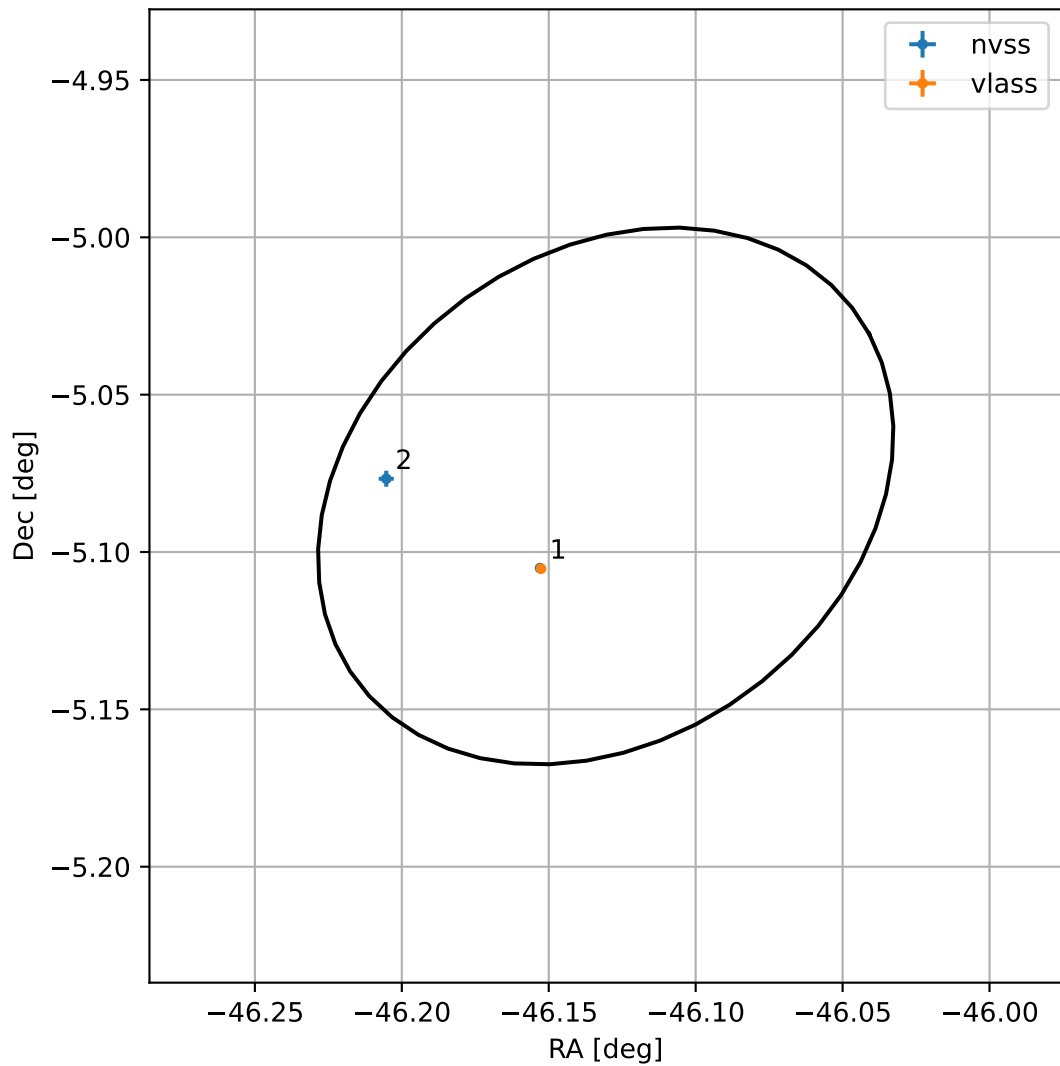
4FGL J2055.4-0504
