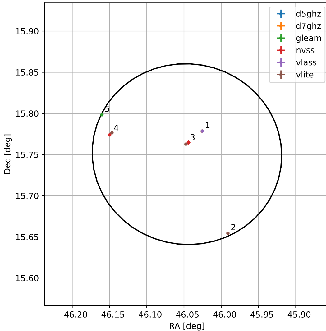
4FGL J2055.8+1545
