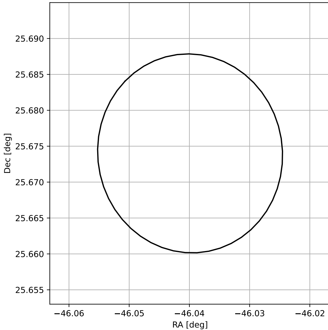
4FGL J2055.8+2540
