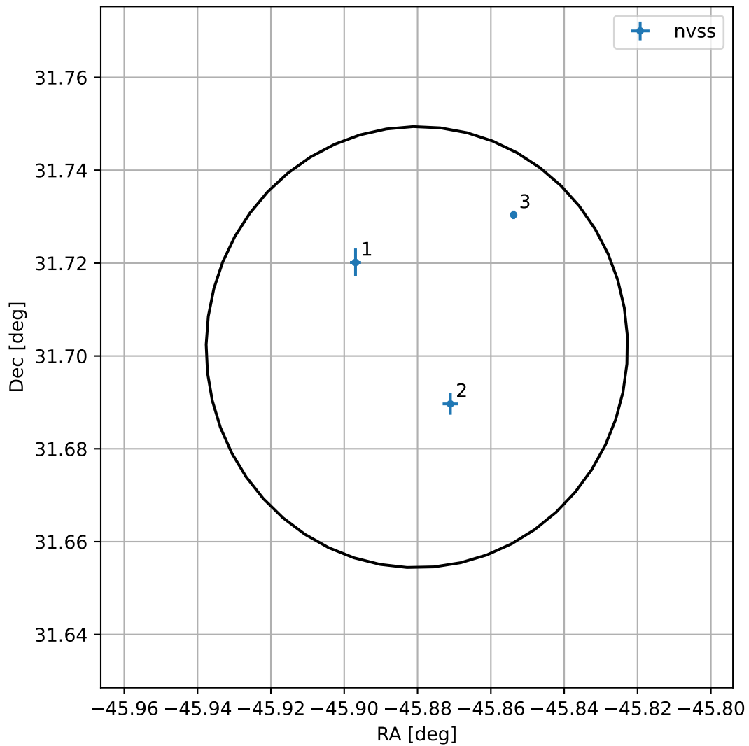
4FGL J2056.4+3142
