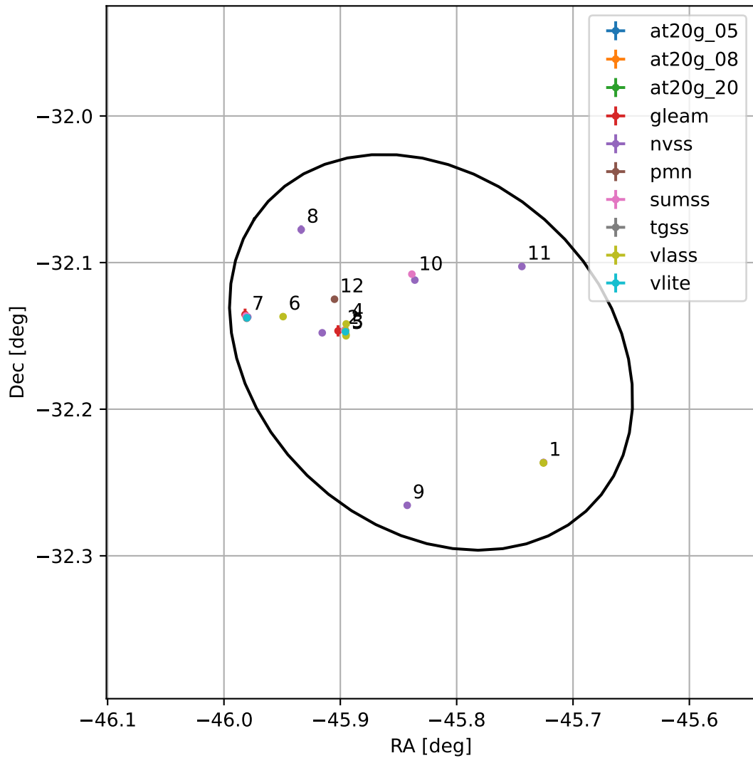
4FGL J2056.7-3209
