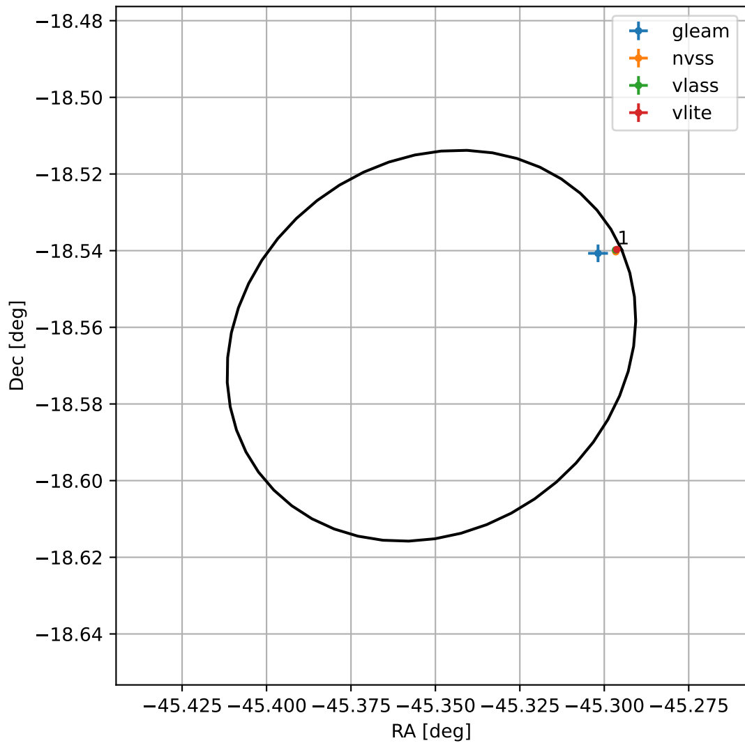
4FGL J2058.5-1833
