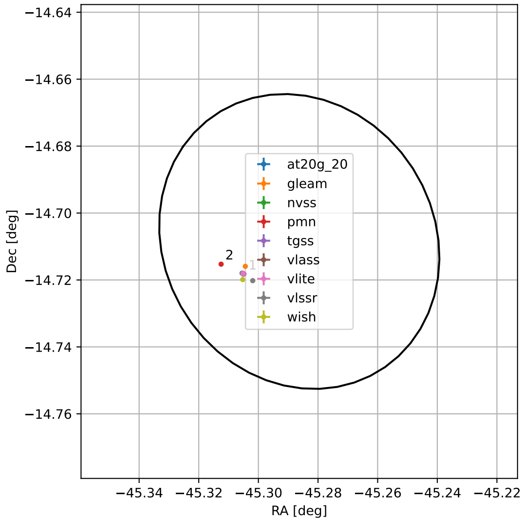
4FGL J2058.8-1442
