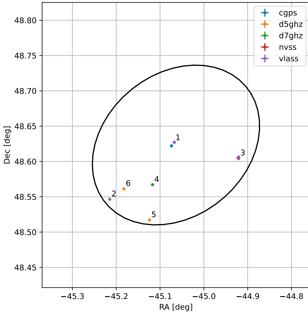
4FGL J2059.7+4837
