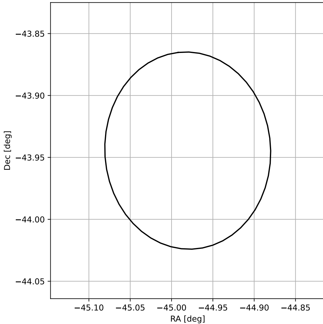
4FGL J2100.0-4356
