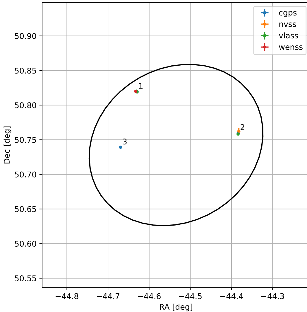
4FGL J2101.8+5044
