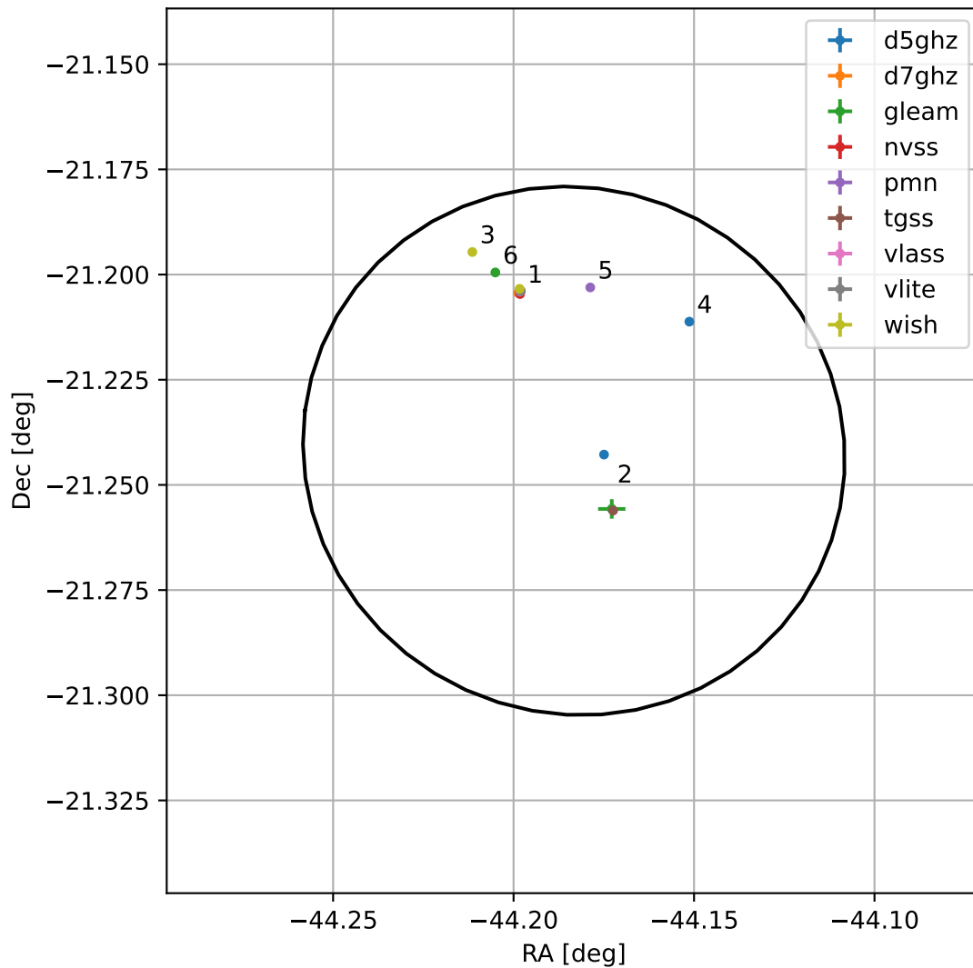
4FGL J2103.2-2114
