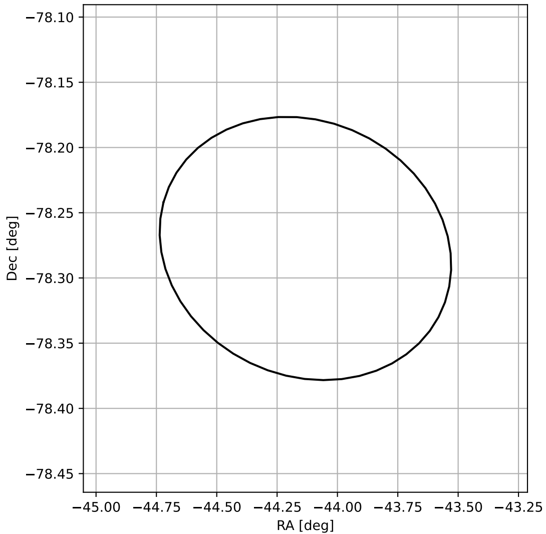
4FGL J2103.4-7816
