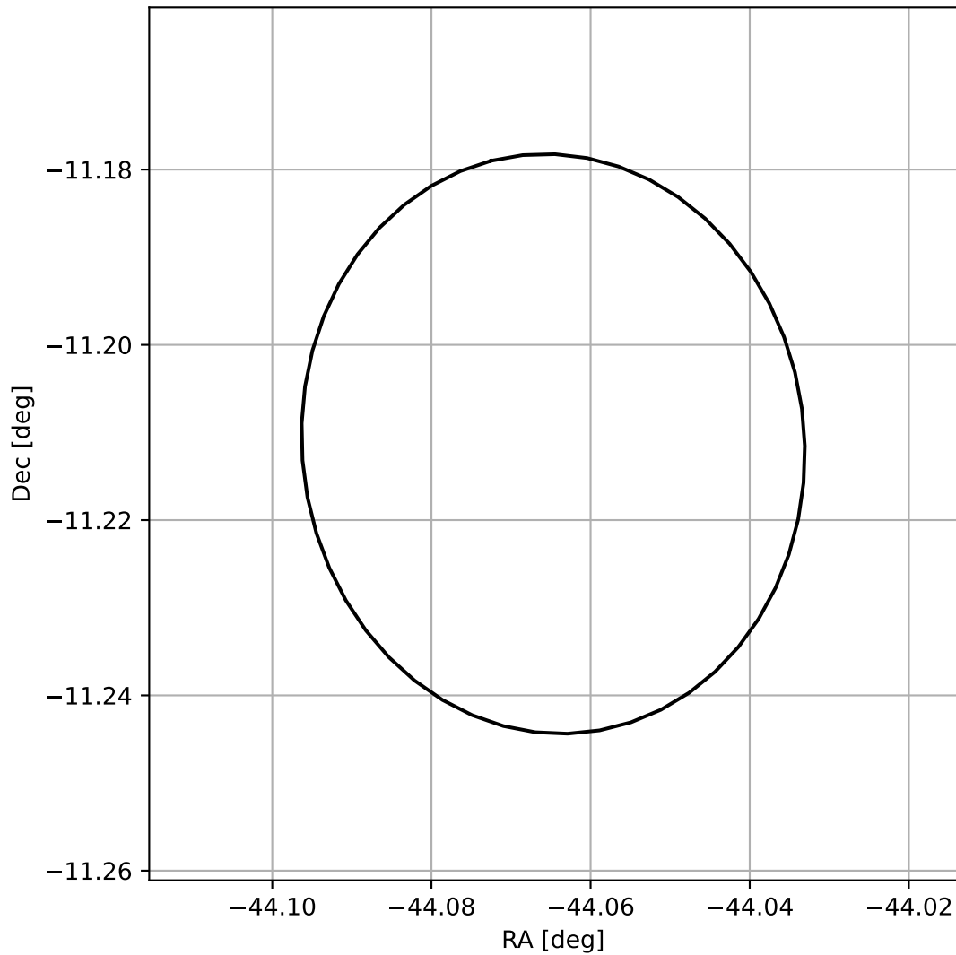
4FGL J2103.7-1112
