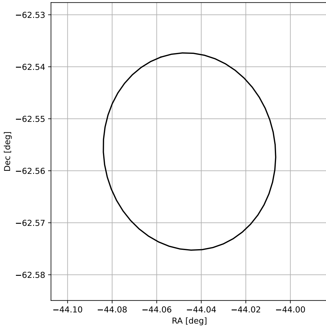
4FGL J2103.8-6233
