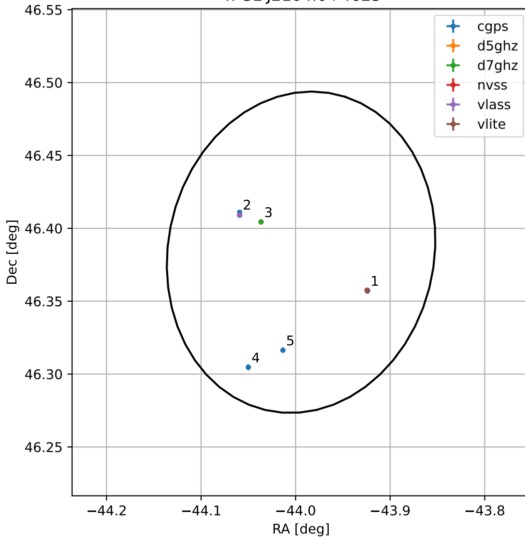
4FGL J2104.0+4623
