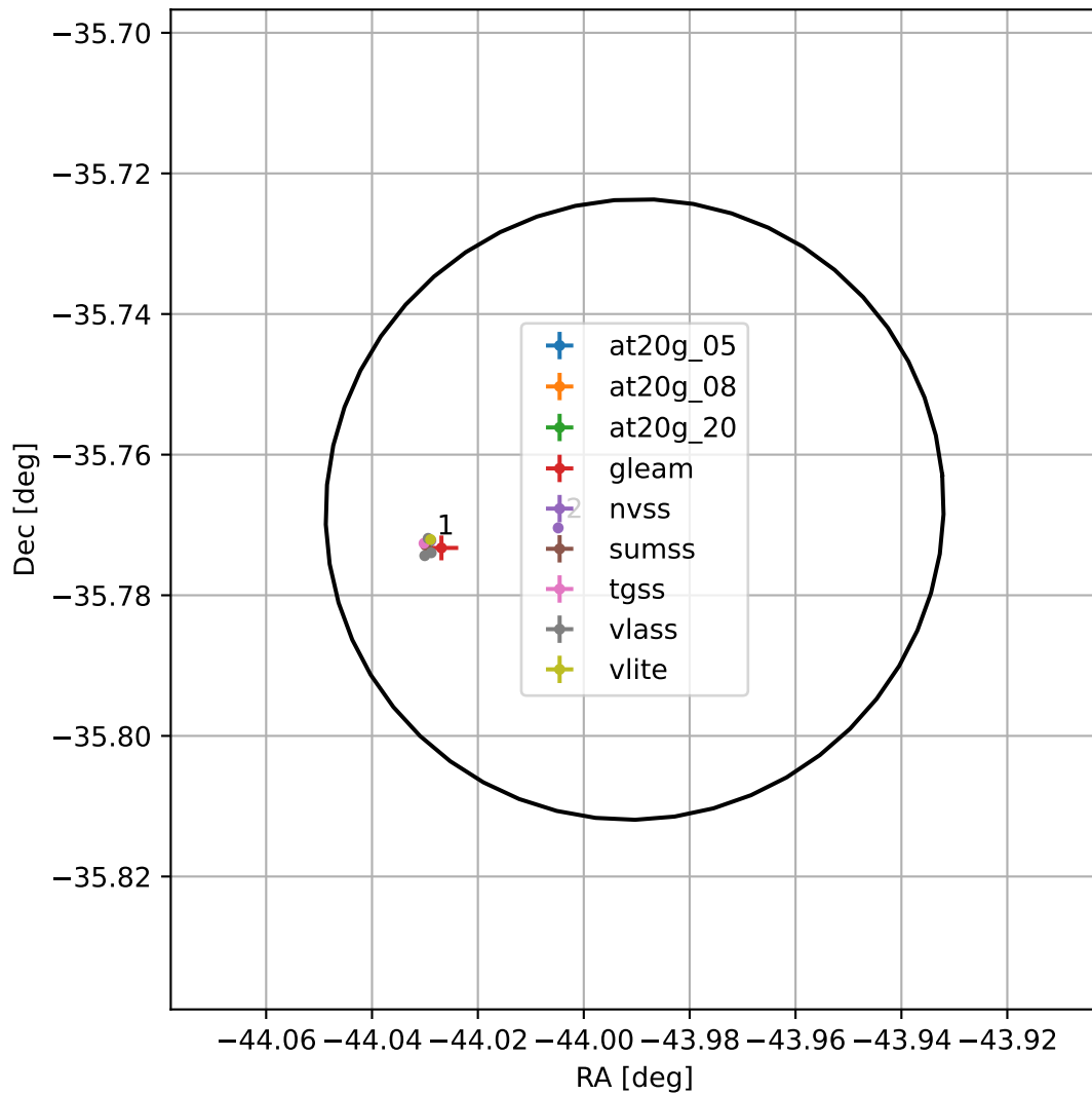
4FGL J2104.0-3546
