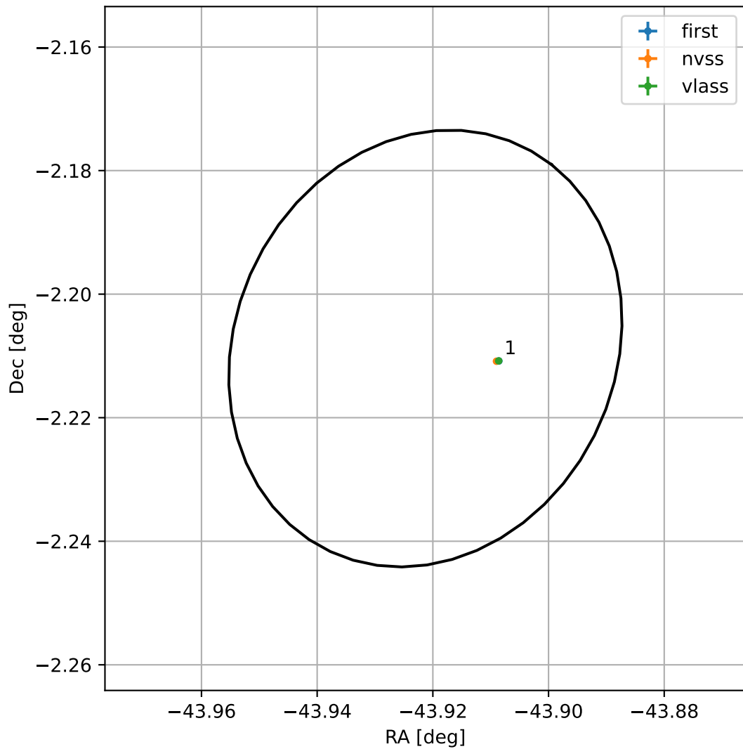
4FGL J2104.3-0212
