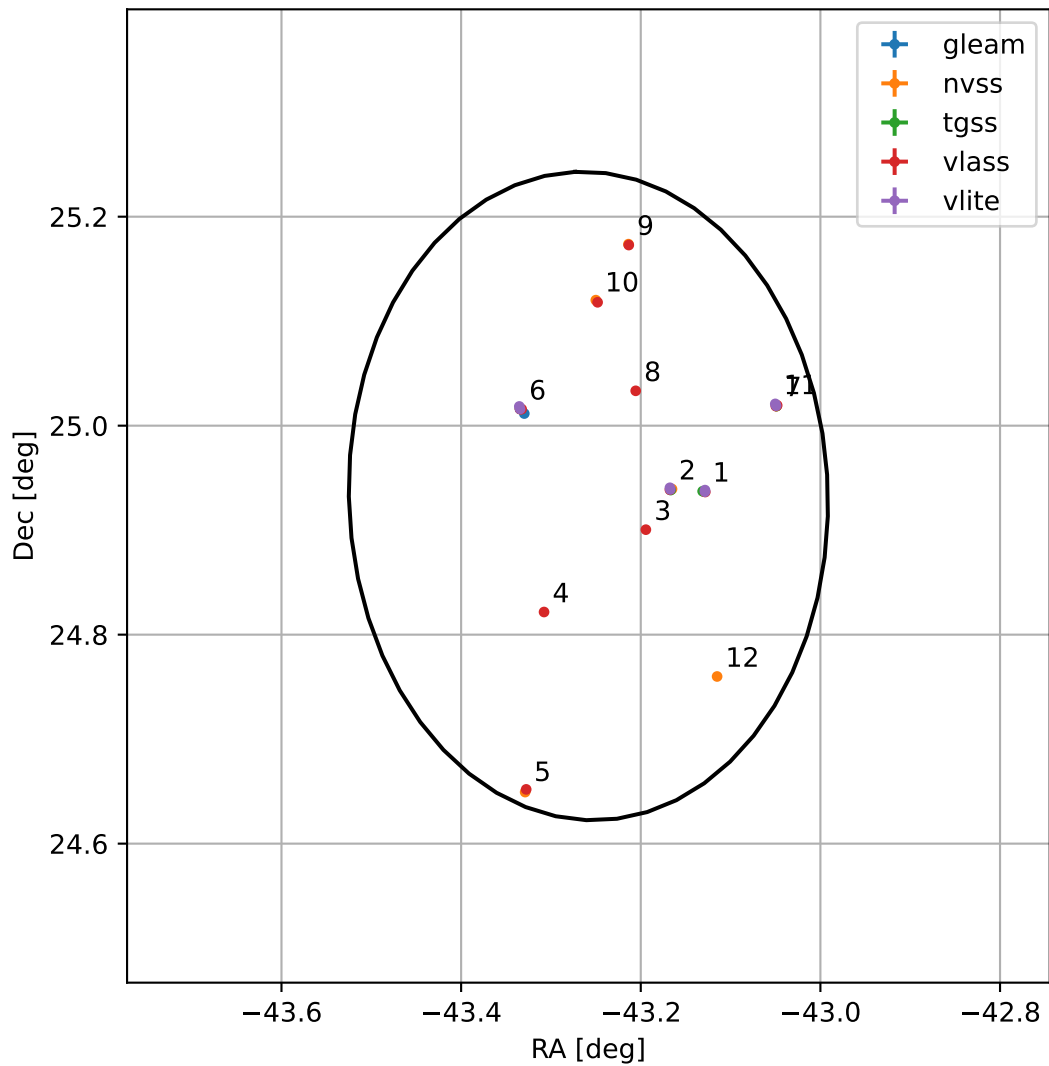
4FGL J2106.9+2455
