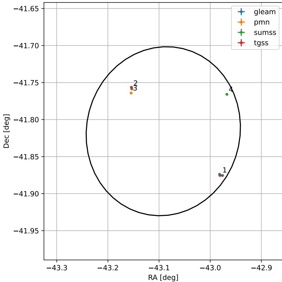
4FGL J2107.6-4148
