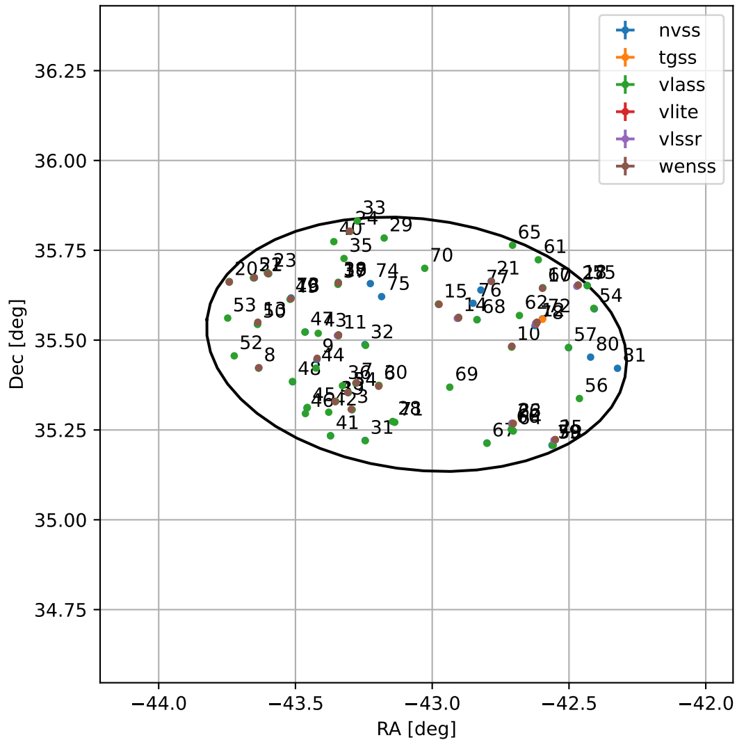
4FGL J2107.7+3529
