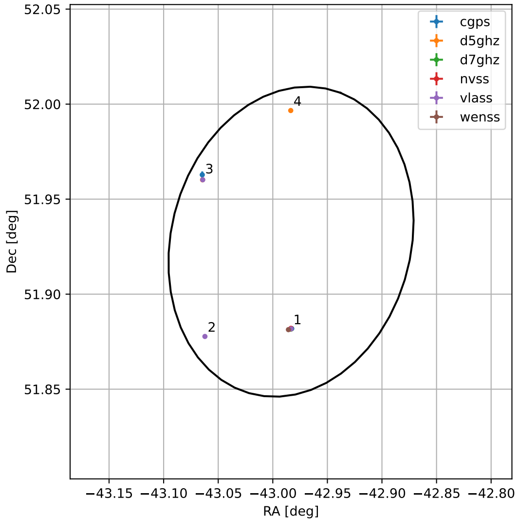
4FGL J2108.0+5155
