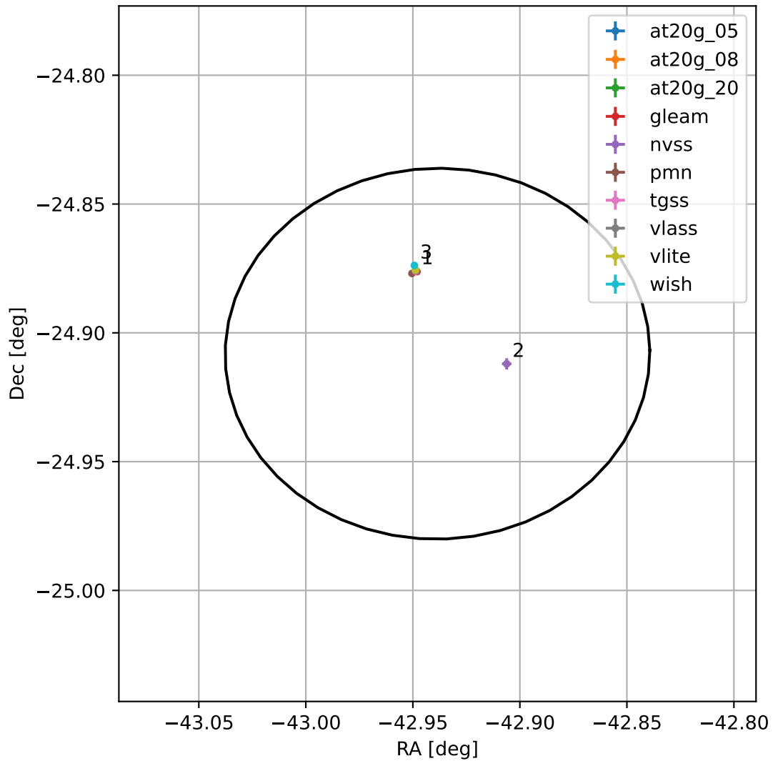
4FGL J2108.2-2454
