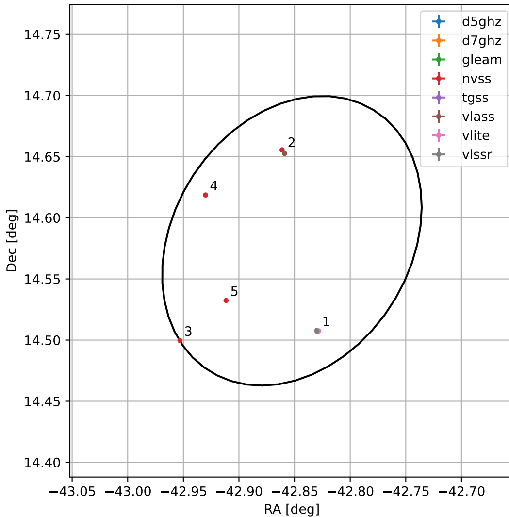
4FGL J2108.5+1434
