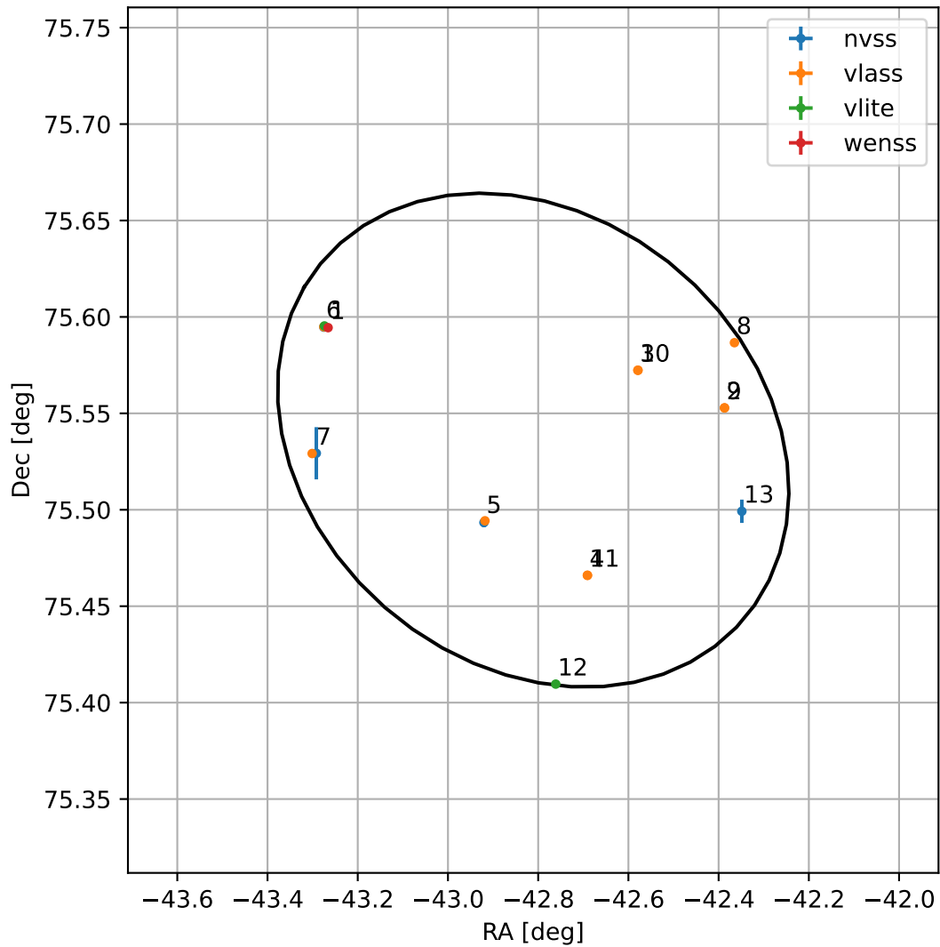
4FGL J2108.7+7532
