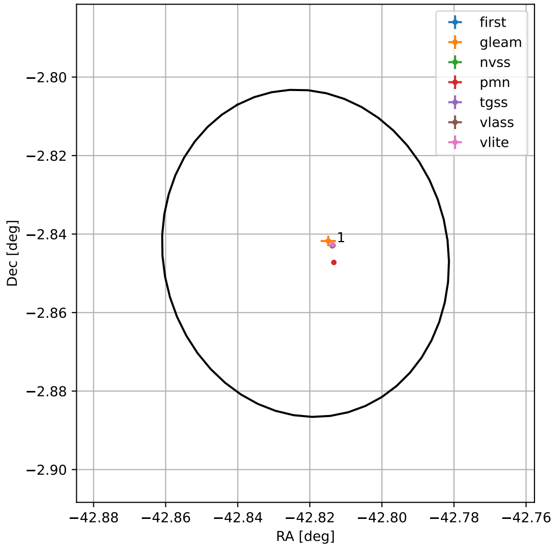
4FGL J2108.7-0250
