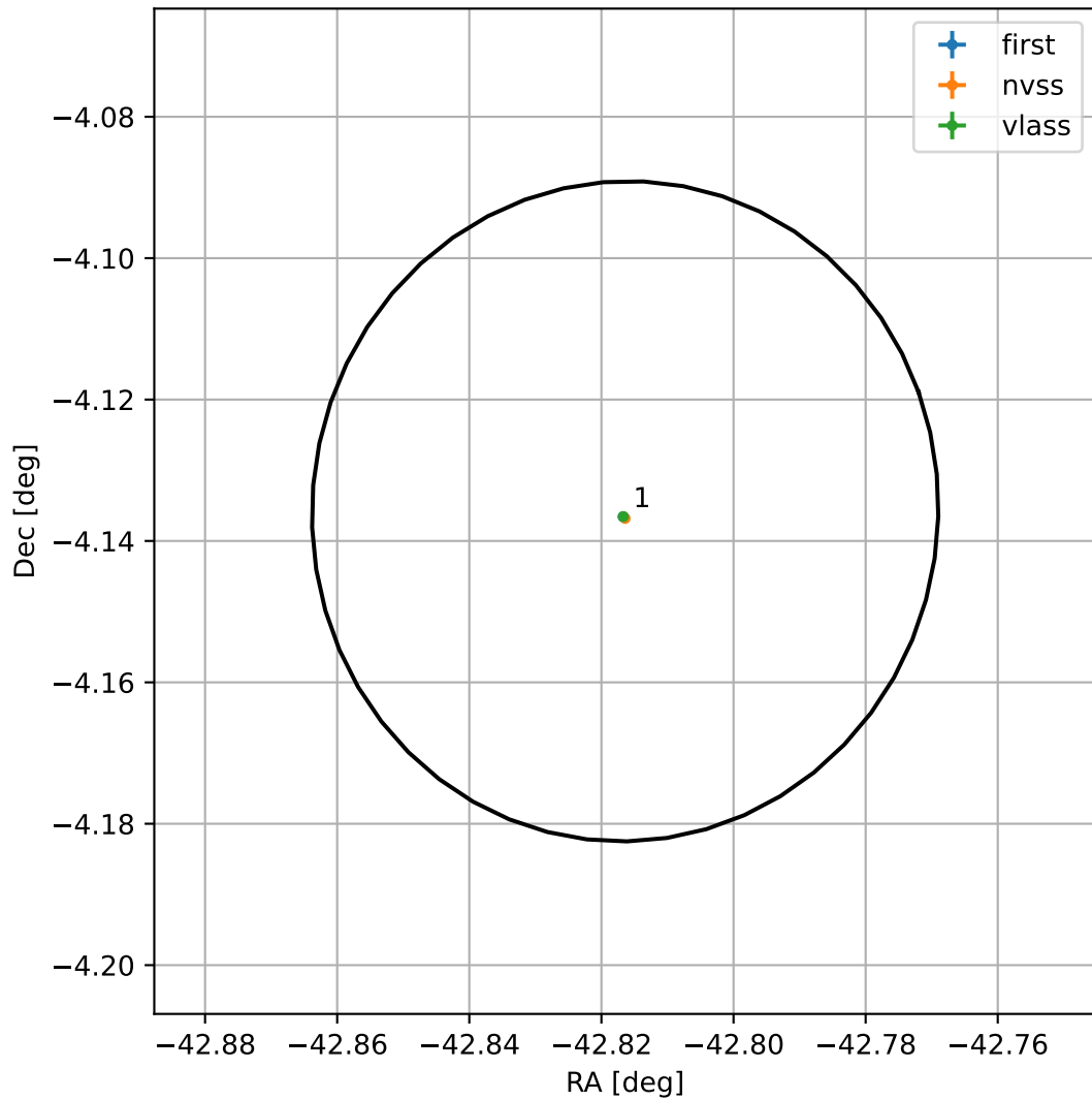
4FGL J2108.7-0408
