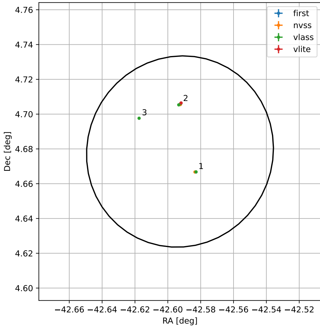
4FGL J2109.6+0440
