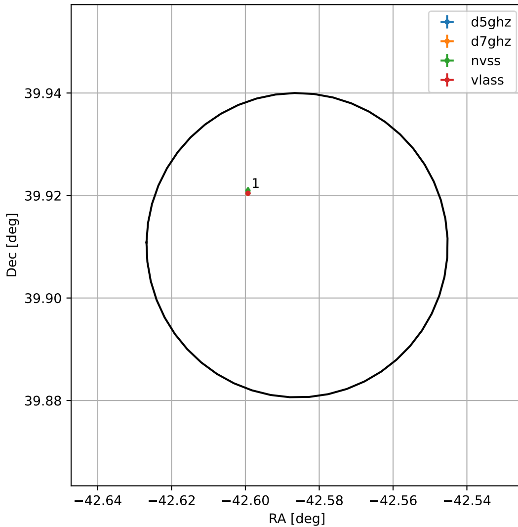
4FGL J2109.6+3954
