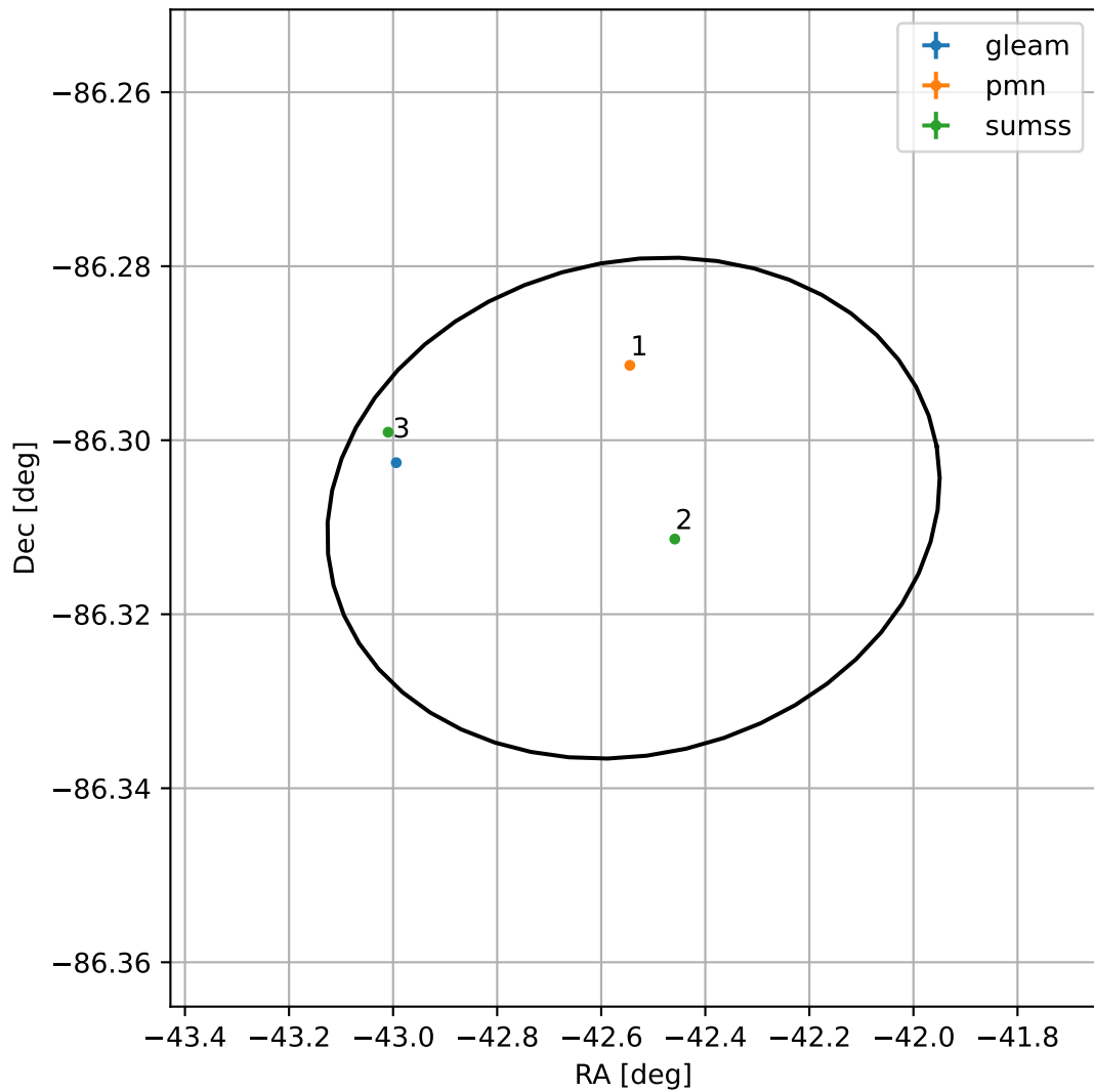
4FGL J2109.8-8618
