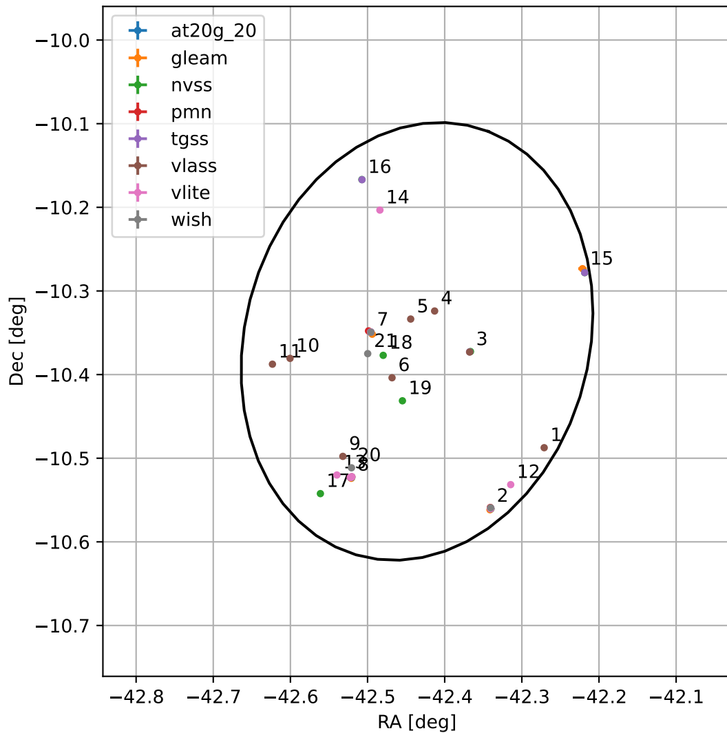
4FGL J2110.2-1021
