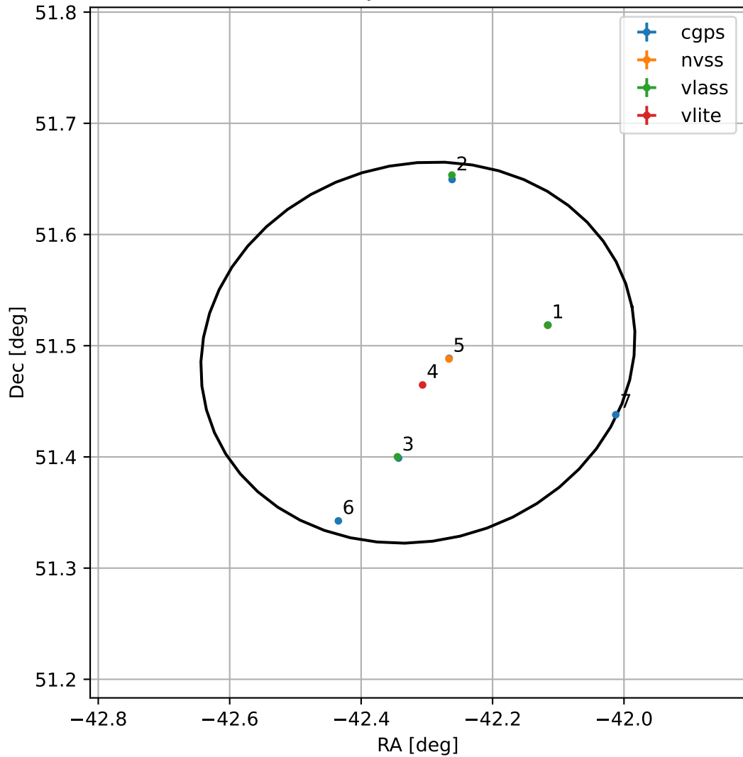
4FGL J2110.7+5129
