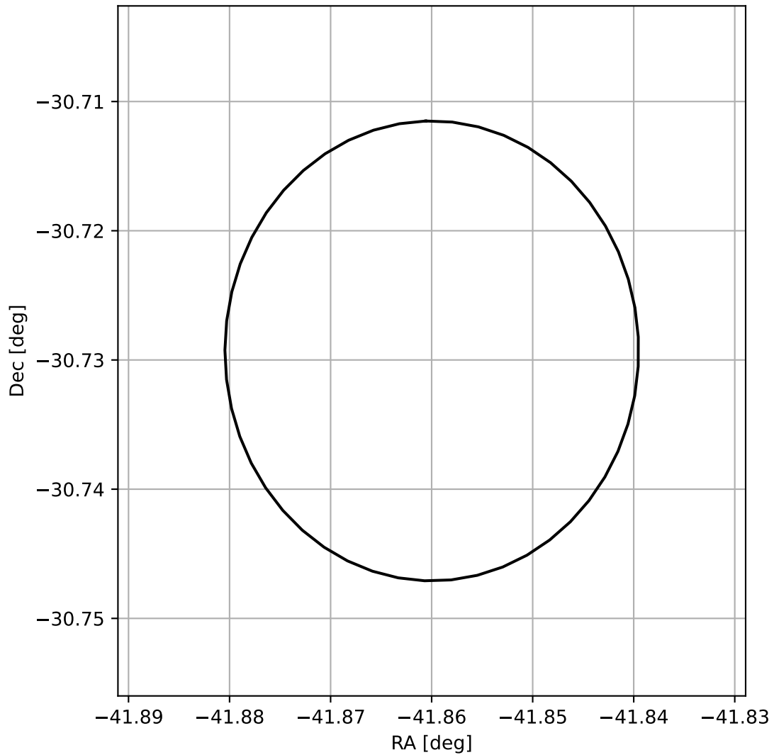
4FGL J2112.5-3043
