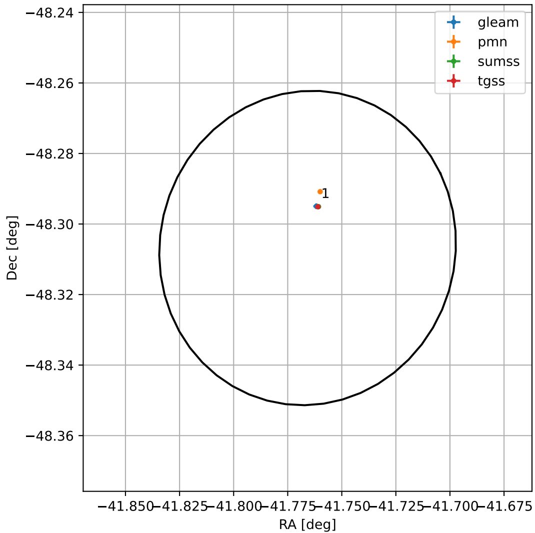
4FGL J2112.9-4818
