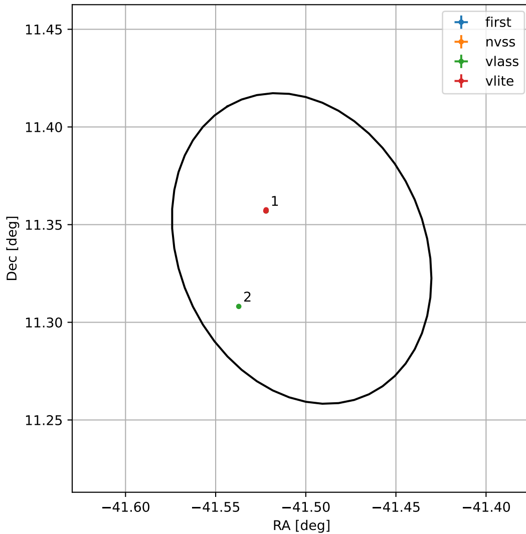
4FGL J2113.9+1120
