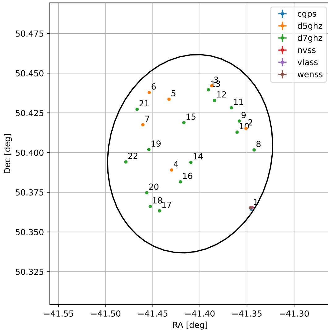
4FGL J2114.3+5023
