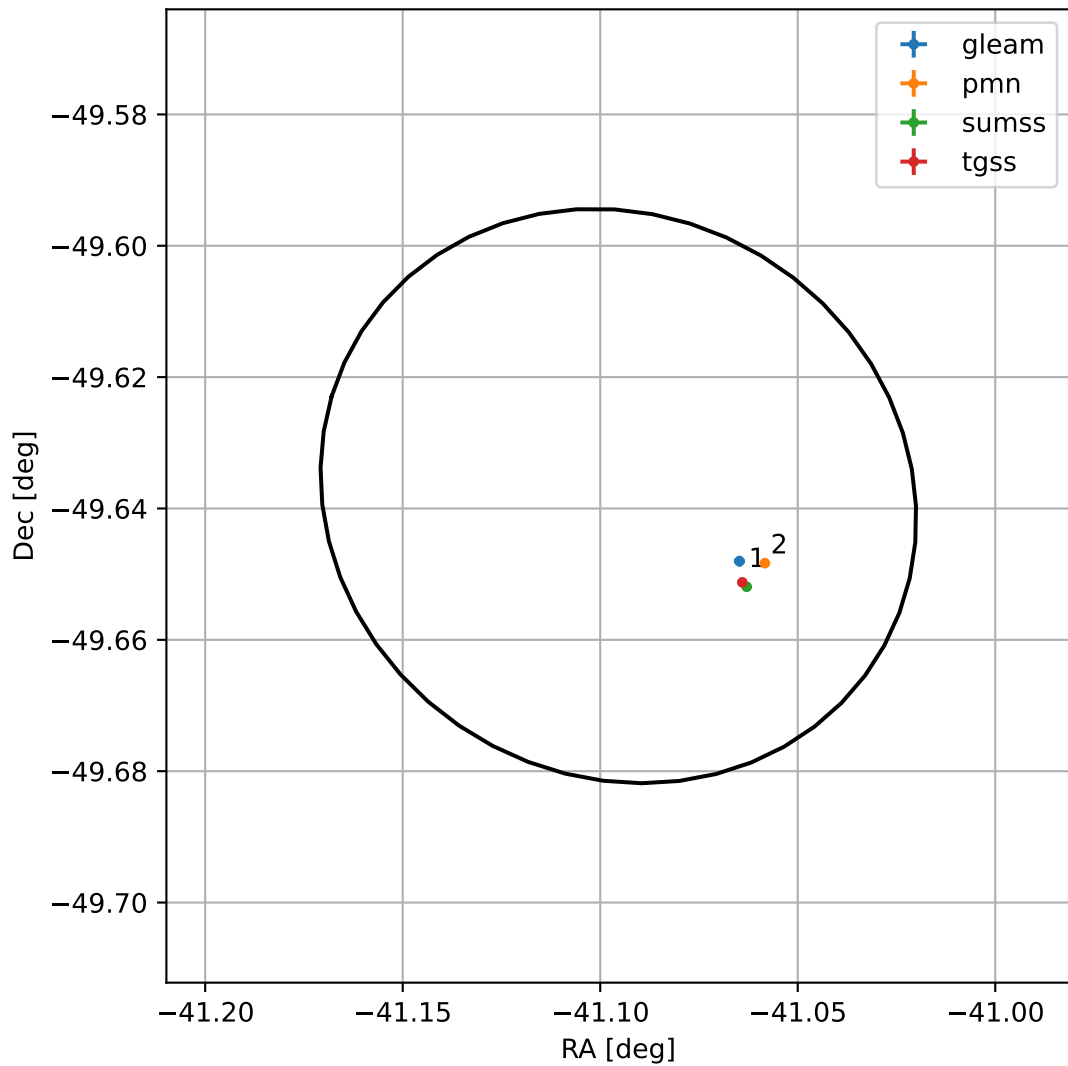
4FGL J2115.6-4938
