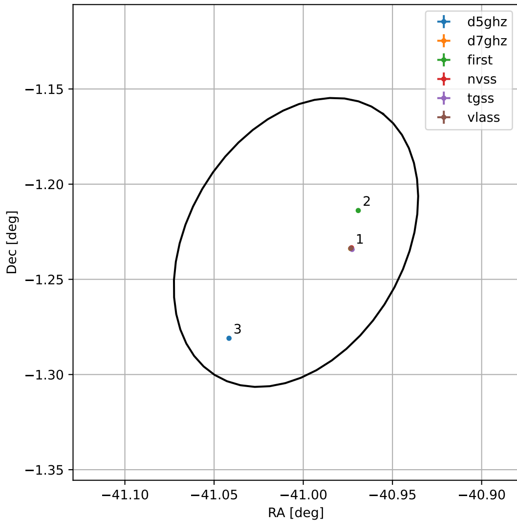
4FGL J2115.9-0113
