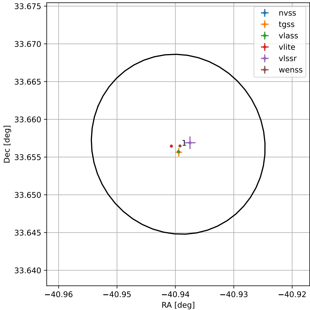
4FGL J2116.2+3339
